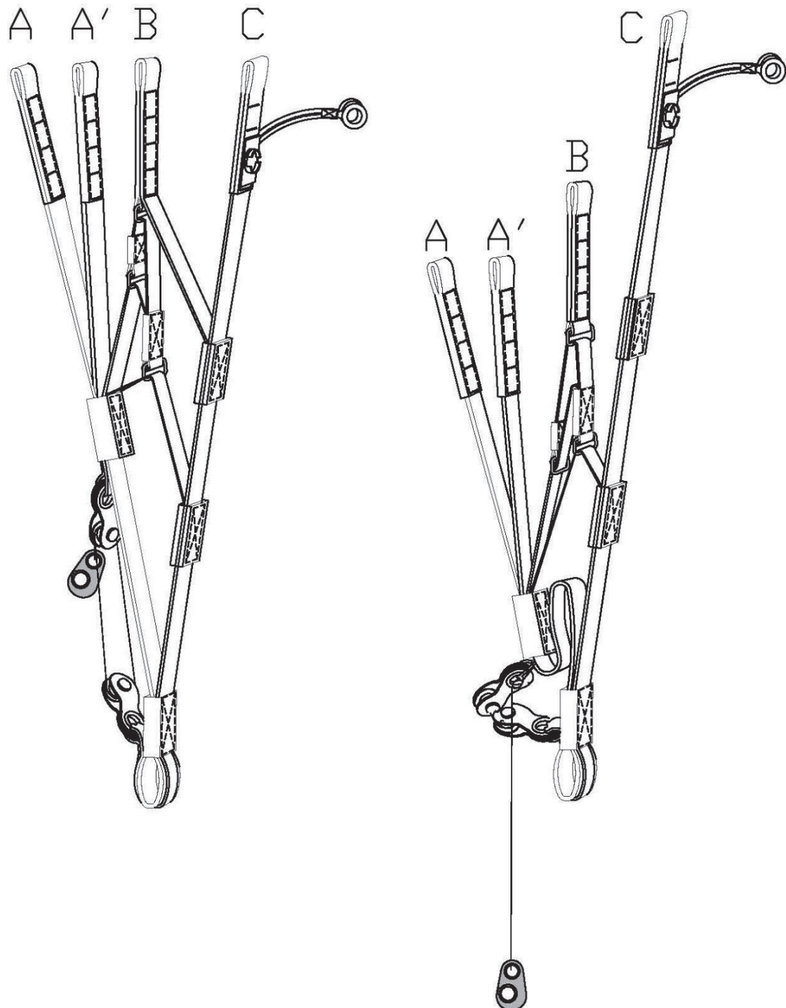
Figure: Atlas 2 riser
